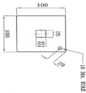
Drawing (No.1)
