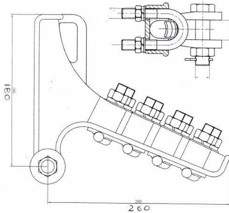
body of TENSION CLAMP
