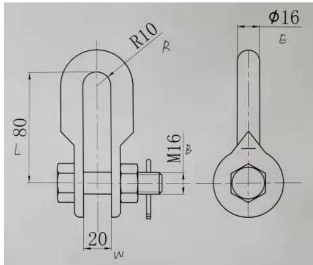
Dimension of D-SHACKLE
