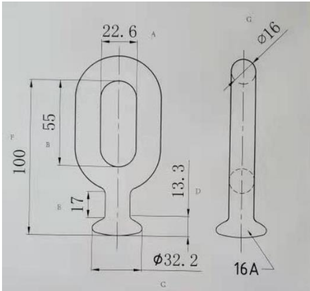
Dimension of BALL EYE
