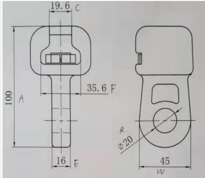
Dimension of SOCKET TONGUE
